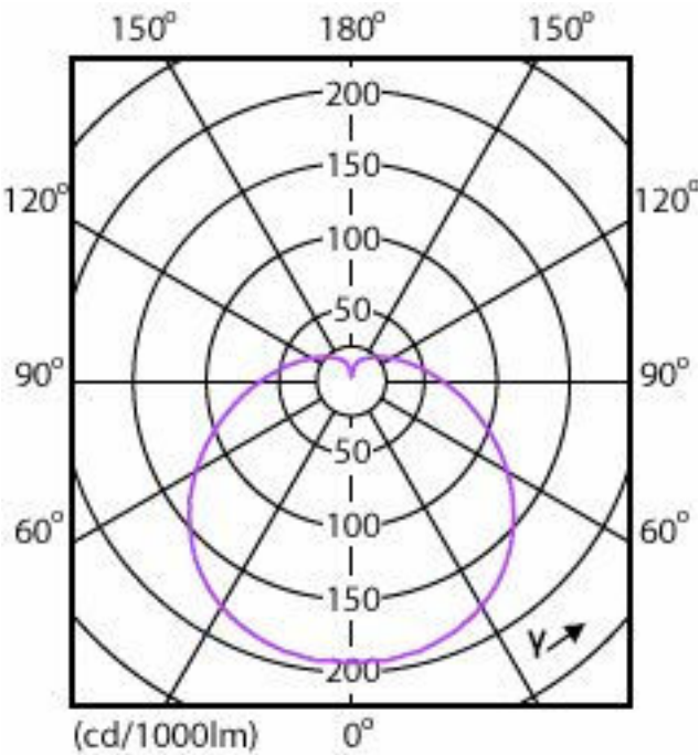
Light Distribution Diagram - EcoHome LEDBulb 6W E27 3000KHV 1PF/20AR
