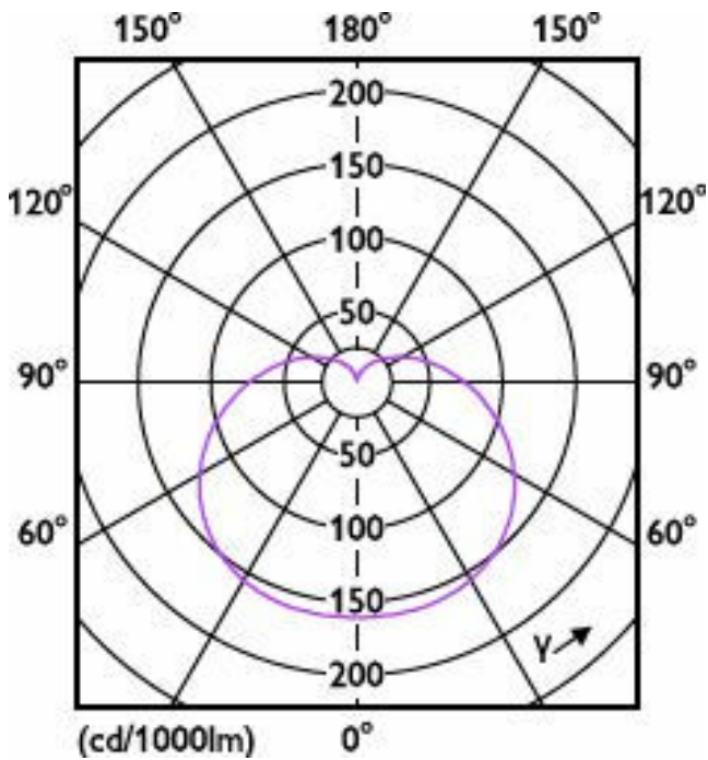
Light Distribution Diagram - EcoHome LEDBulb 4W E27 3000K G45 1PF AR
