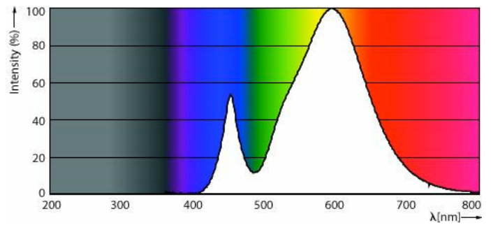
Spectral Power Distribution Colour - EcoHome LEDBulb 4W E27 3000K G45 1PF AR
