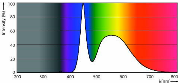
Spectral Power Distribution Colour - EcoHome LEDBulb 4W E27 6500K G45 1PF AR
