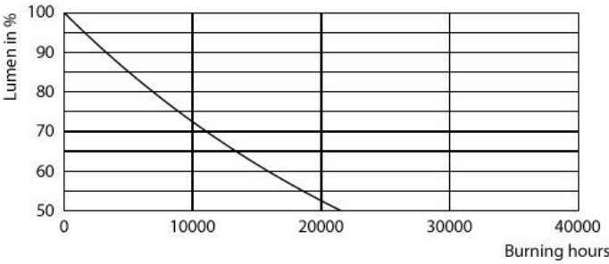
Lumen Maintenance Diagram - EcoHome LEDBulb 4W E27 6500K G45 1PF AR
